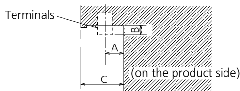
Terminal b 65SF2W Terminal (Bottom)
