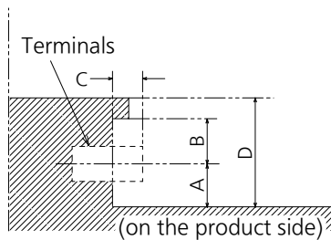
Sectional view of terminal b (USB / LAN / IR IN / IR OUT / HDMI 1 / HDMI 2)
