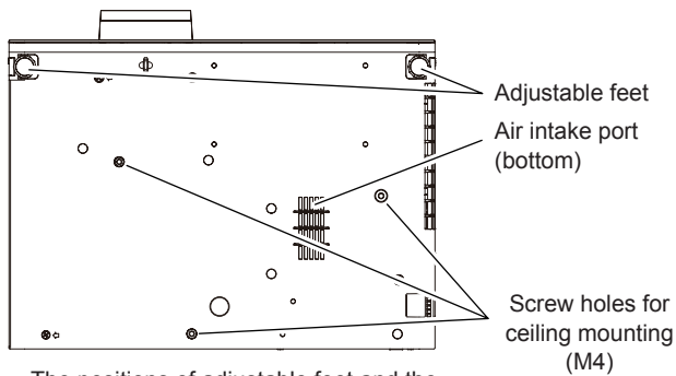
The positions of adjustable feet and the screw holes for ceiling mounting
