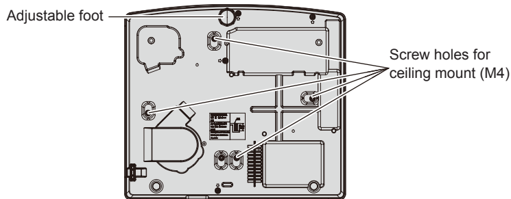
Positions of screw holes for ceiling mount and adjustable foot
