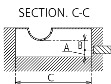
Sectional view of terminal c (USB TYPE-A)
