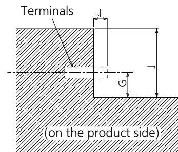
Sectional view of terminal b (USB/LAN/SERIAL)
