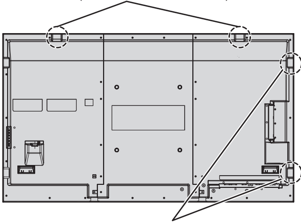
Eyebolt mounting positions (for vertical installation)
