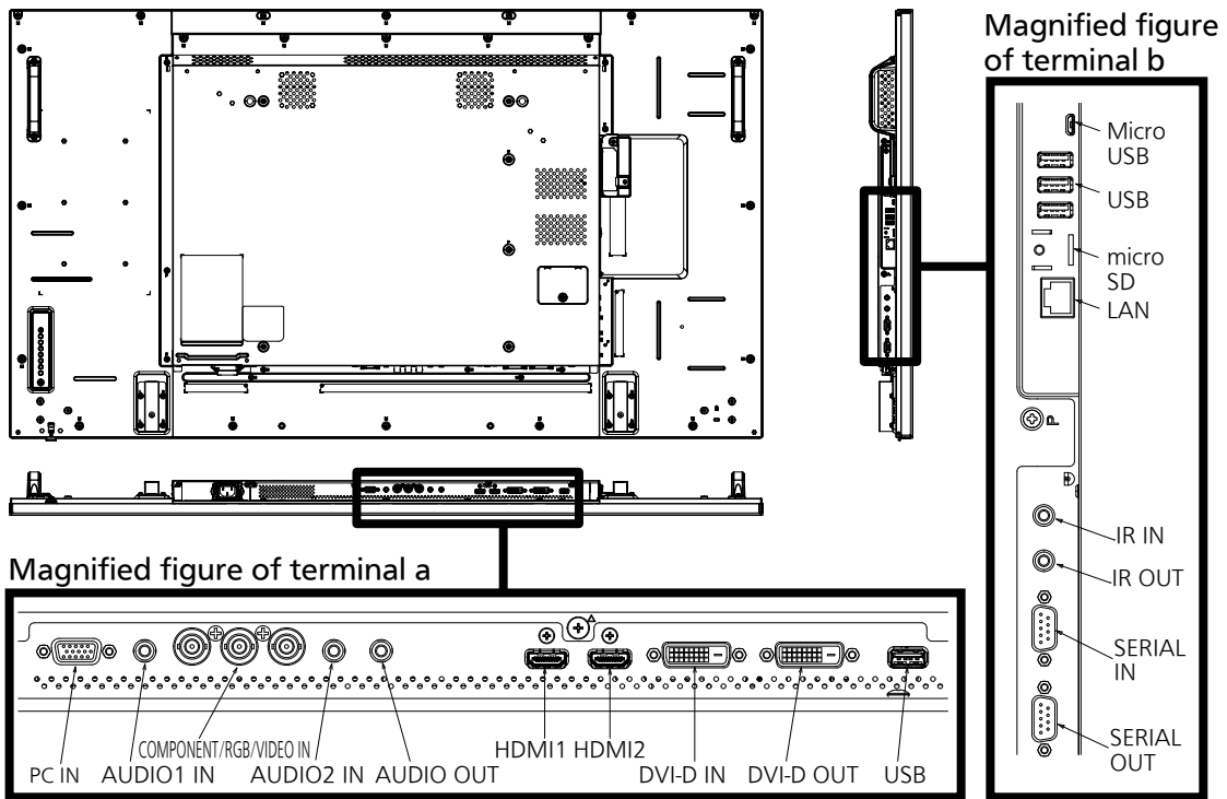
Sectional view of terminal a (PC/AUDIO/COMPONENT/HDMI/DVI-D IN/USB)
