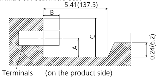
Terminal b 55AF1 Terminal (Side)
