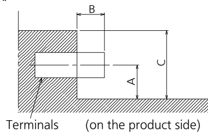
Sectional view of terminal b (SERIAL/IR)
